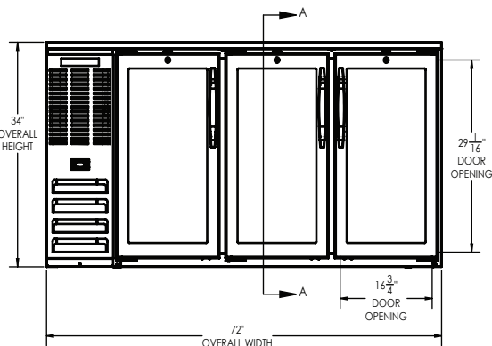
ELEVATION VIEW
