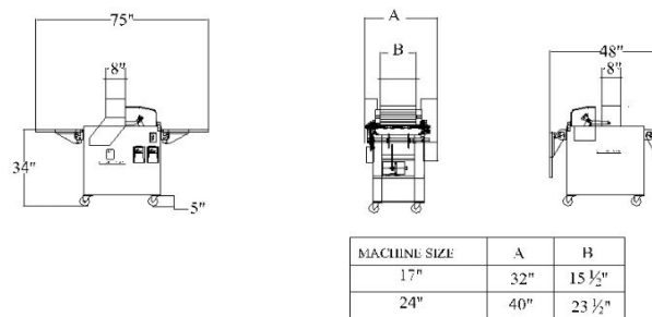
17 V & 24 V COOKIE DEPOSITOR DIMENSION DIAGRAM
