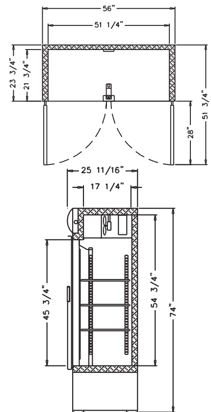
TOP VIEWS AND SIDE VIEWS
