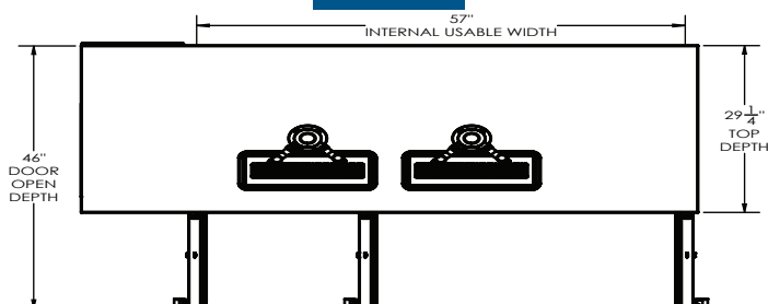
PLAN VIEW
