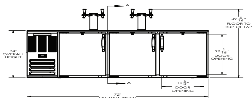
ELEVATION VIEW
