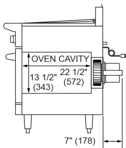
Side Convection with 26-1/2" Oven Base
