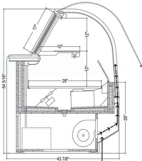
FRONT AIR CHASER FLOW
