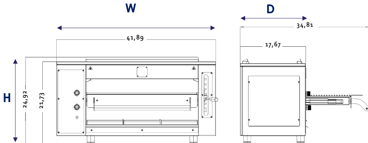
FRONT VIEW (Door Closed)
