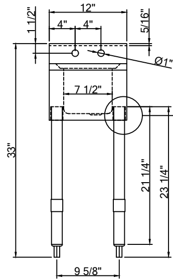
FRONT ELEVATION
