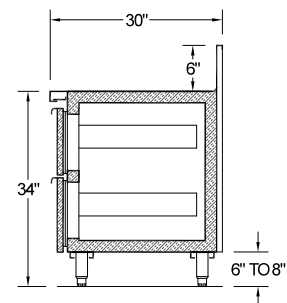
SECTION VIEW
