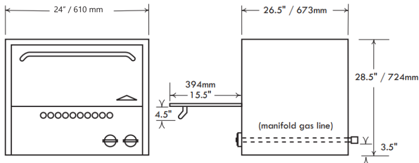
Model PO19 - 300 lbs. / 136 Kgs.
