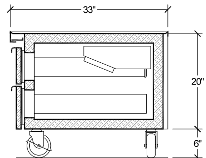
SECTION VIEW
