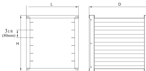
TSP-2224-V FRONT VIEW
