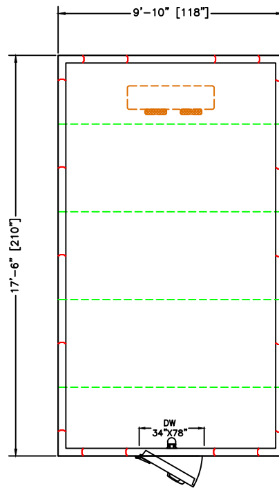
PLAN VIEW
