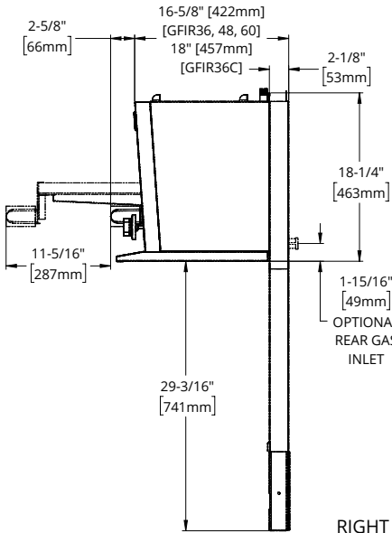
RIGHT VIEW
