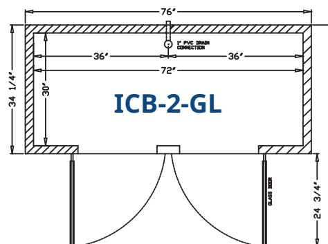
PLAN VIEWS
