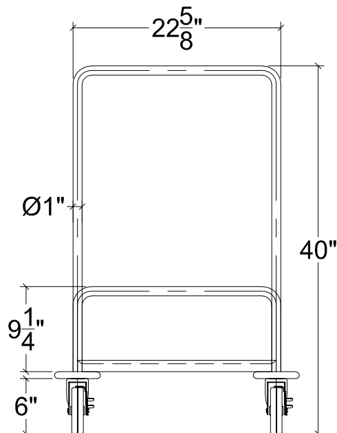
(A) ELEVATION
