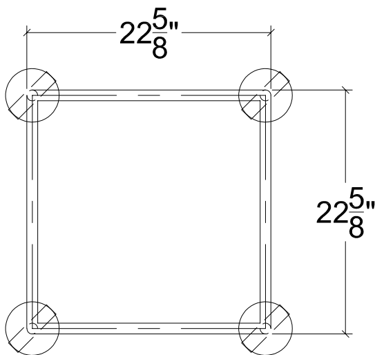
(A) PLAN
