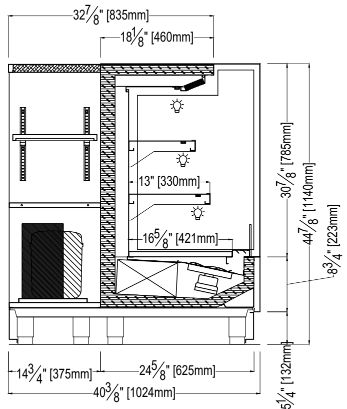
MURO H11-2: SELF CONTAINED RM W/ BACK SHELVEING
