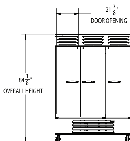
ELEVATION VIEW
