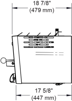
SIDE
