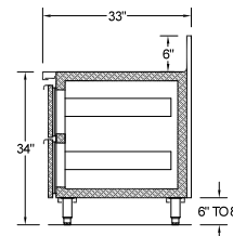
SECTION VIEW
