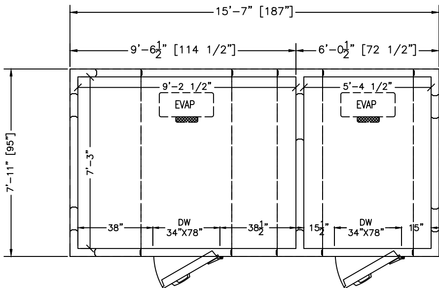
COOLER (WITH FLOOR PANELS)
