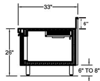
SECTION VIEW
