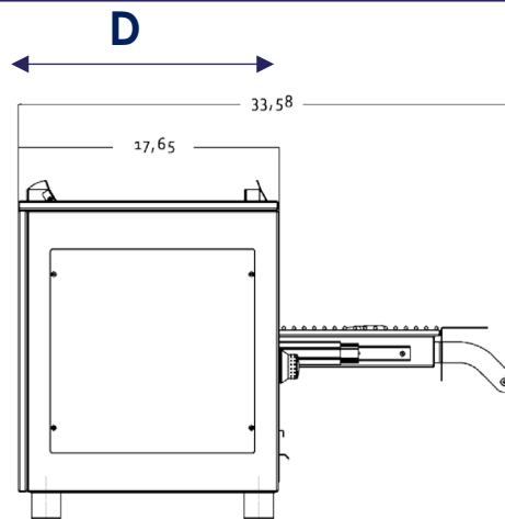
SIDE VIEW (Door Open)
