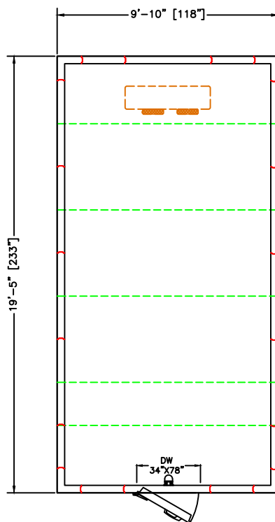
PLAN VIEW
