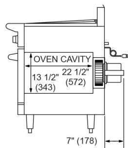
Side Convection with 26-1/2" Oven Base
