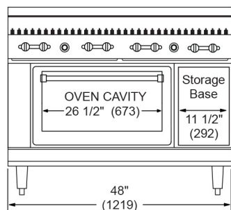
Front AR-4RB with 26-1/2" Oven
