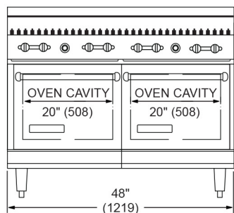
Front AR-4RB with (2) Space Saver Ovens
