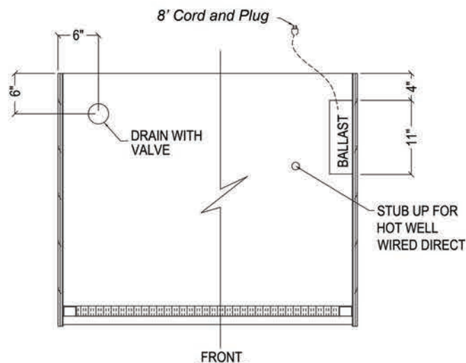
Electrical & Plumbing locations
