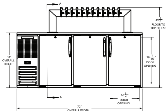
ELEVATION VIEW
