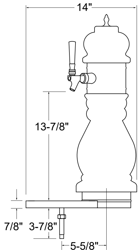
SIDE ELEVATION
