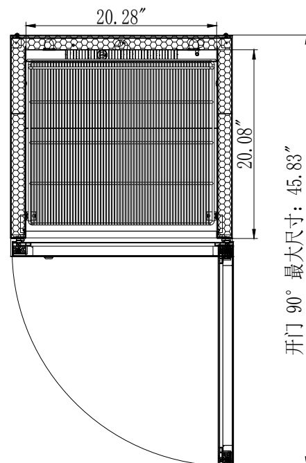
Top View
