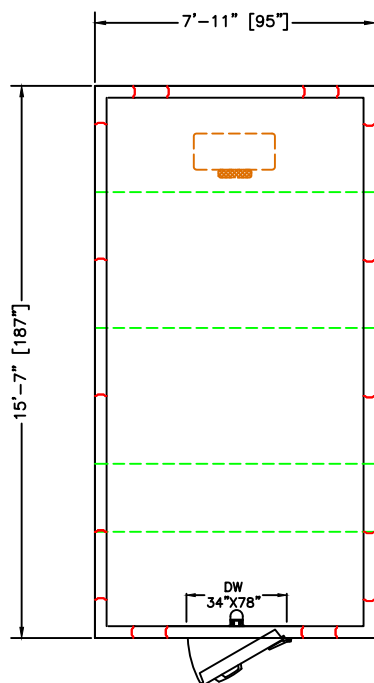
PLAN VIEW RIGHT HINGE SELECT
