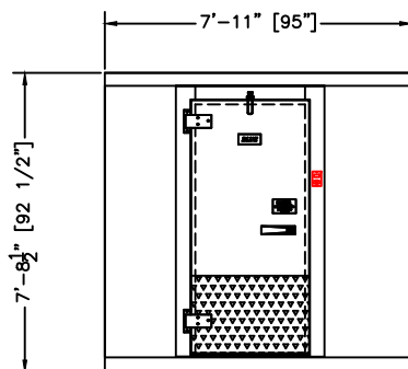
ELEVATION LEFT HINGE
