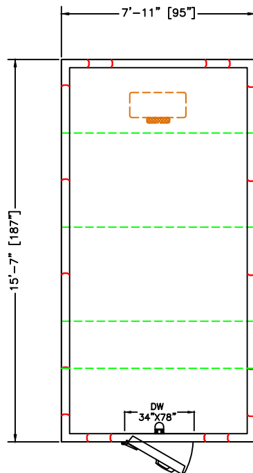
PLAN VIEW LEFT HINGE SELECT
