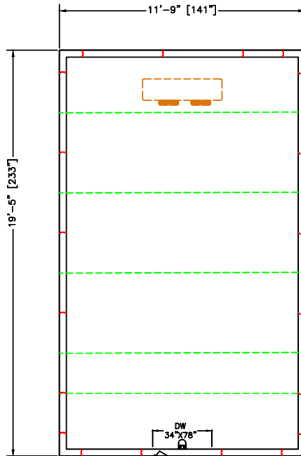
PLAN VIEW LEFT HINGE SELECT
