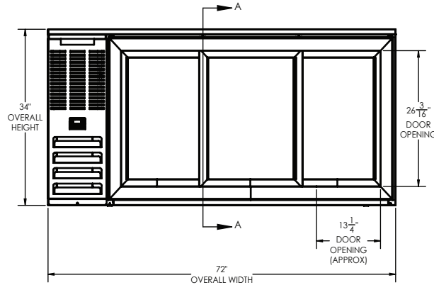
ELEVATION VIEW
