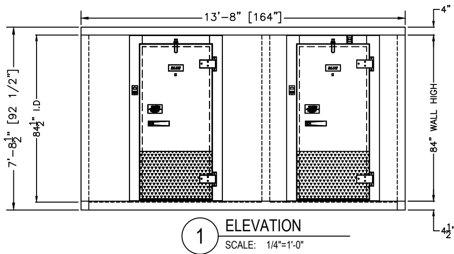
FREEZER (WITH FLOOR PANELS)
