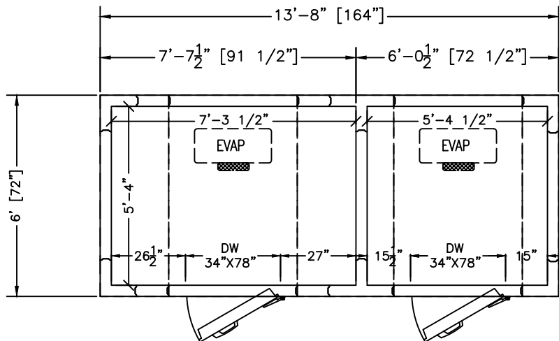
COOLER (WITH FLOOR PANELS)
