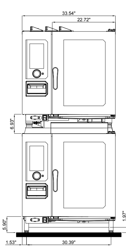
61G + 61G on CHEF-6NLEG1 Stand 6" for stacked ovens
