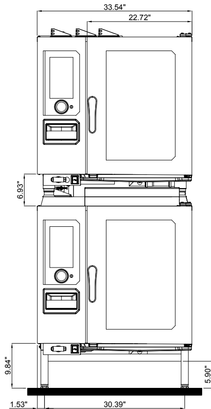
61G + 61G on CHEF-10NLEG1 Stand 10" for stacked ovens
