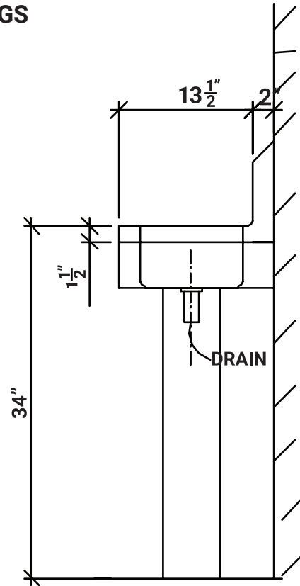
END VIEW
