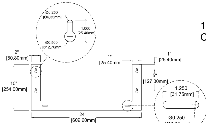
Rear View
