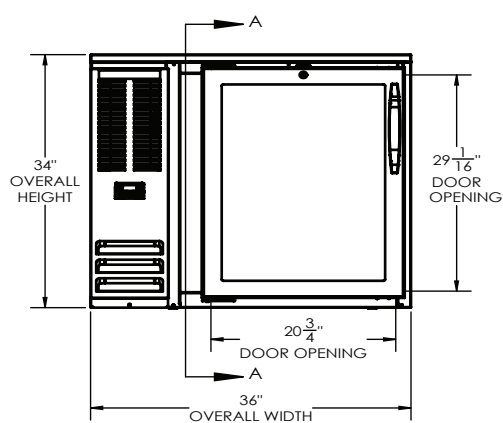
ELEVATION VIEW
