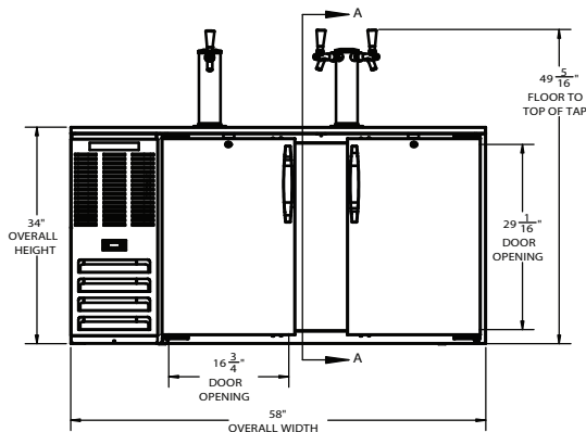
ELEVATION VIEW
