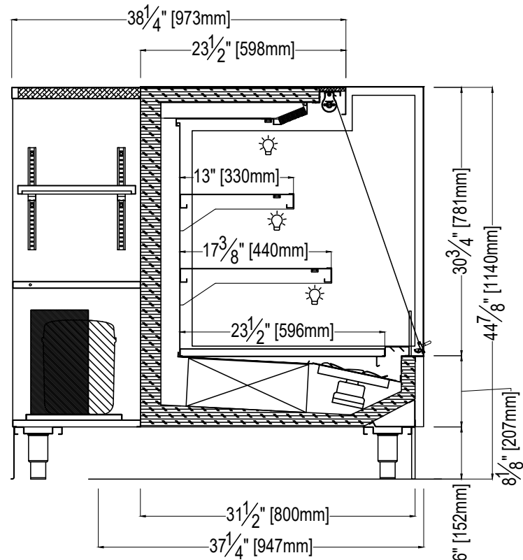
MURO H12-2: SELF CONTAINED RM W/ BACK SHELVEING
