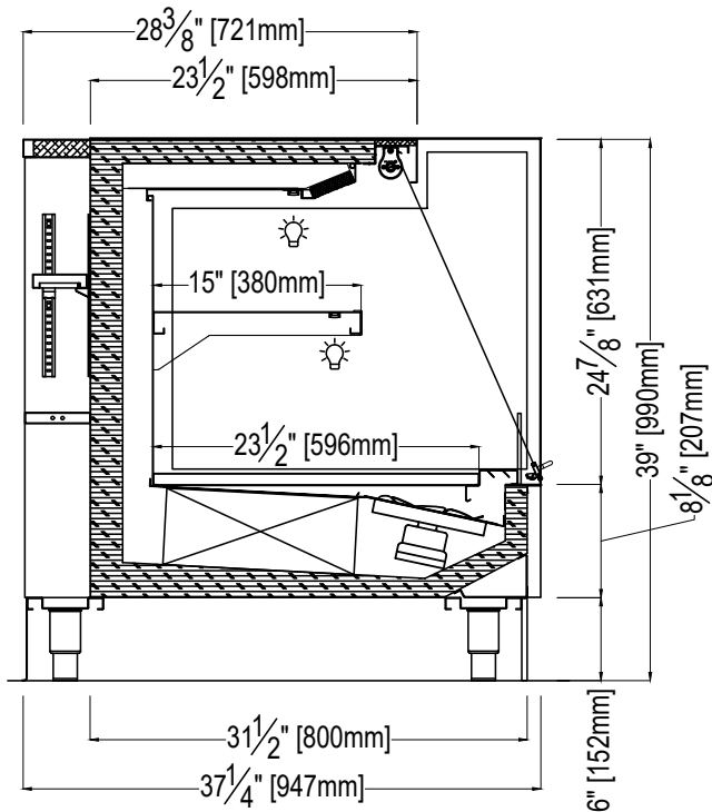
MURO H12-1: REMOTE CONDENSING UNIT W/ BACK SHELVING
