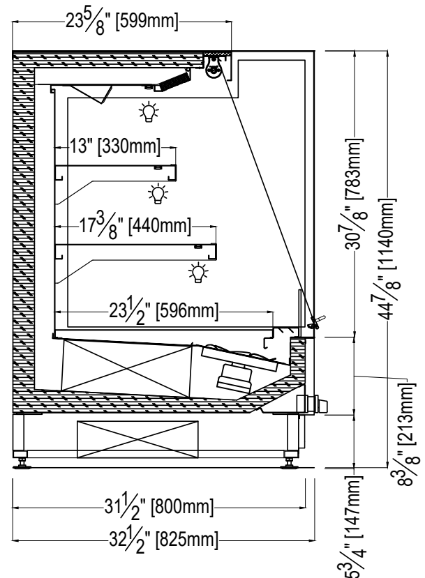
MURO H12-2 REMOTE CONDENSING UNIT
