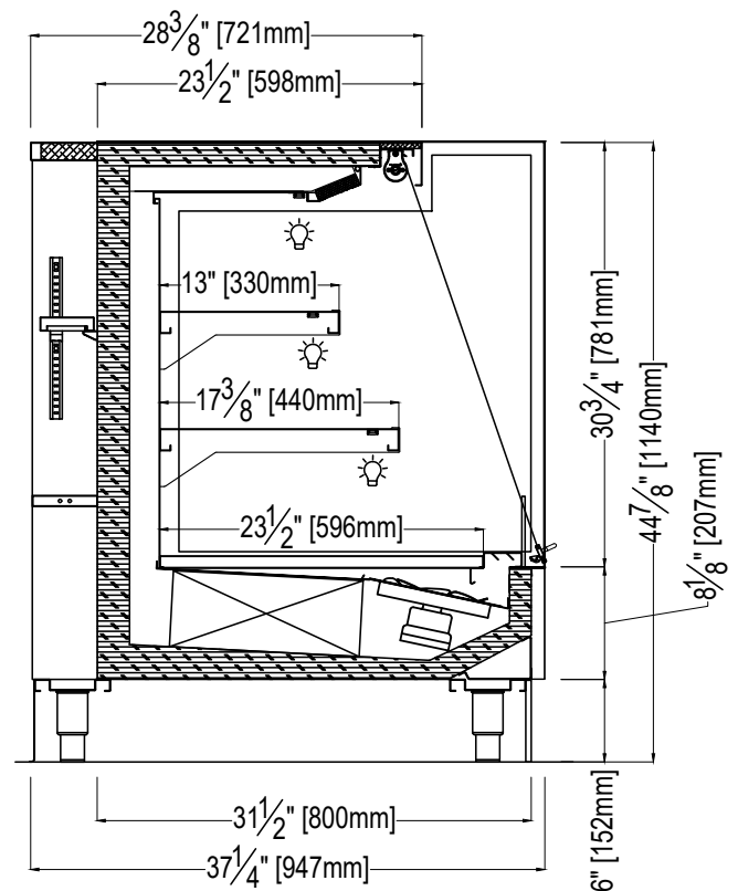
MURO H12-2: REMOTE CONDENSING UNIT W/ BACK SHELVING
