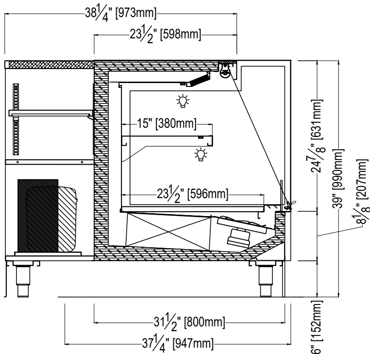
MURO H12-1: SELF CONTAINED RM W/ BACK SHELVEING
