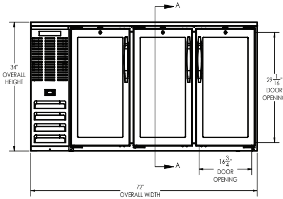
ELEVATION VIEW
