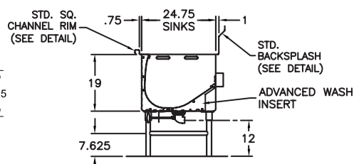
SECTION "A"
