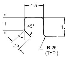
SQ. CHANNEL RIM DETAIL
