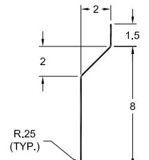
BACKSPLASH DETAIL
