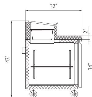
Side Section
