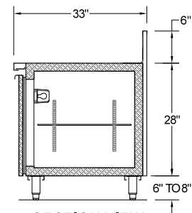
SECTION VIEW
