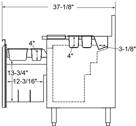
SECTION VIEW
