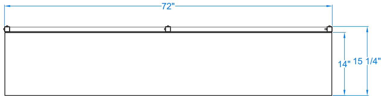
Top View
