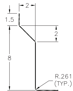
BACKSPLASH DETAIL
