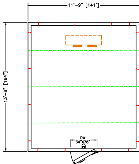
PLAN VIEW
