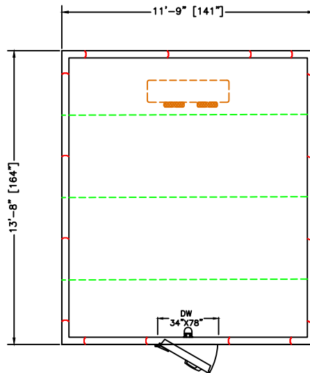
PLAN VIEW
