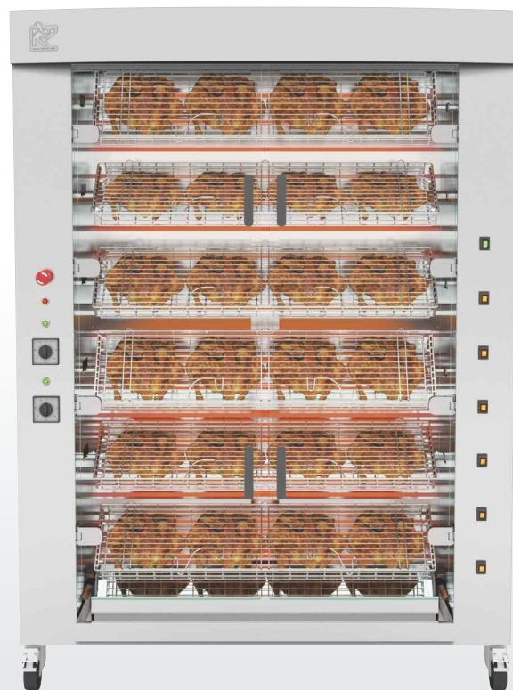
FBS1400-6E-SS Stainless steel & chrome shown with optional roof
