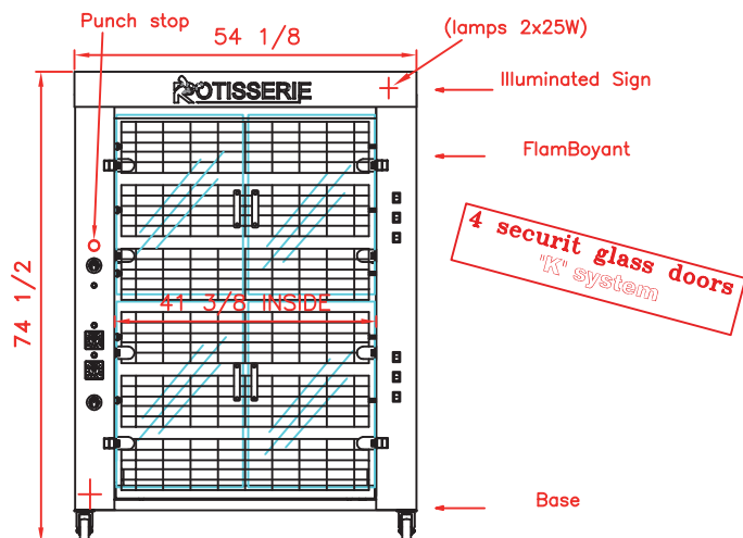
Front view Rotisserie with roof
