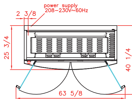
Top view Rotisserie with roof
