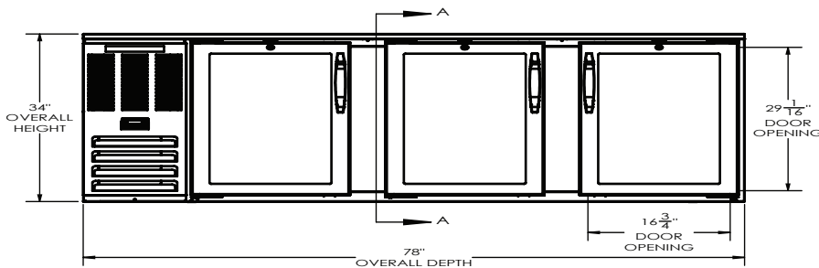
ELEVATION VIEW
