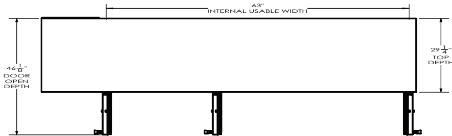
ELEVATION VIEW
