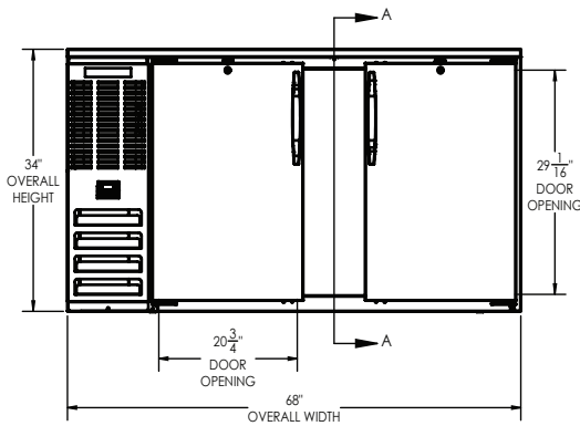
ELEVATION VIEW
